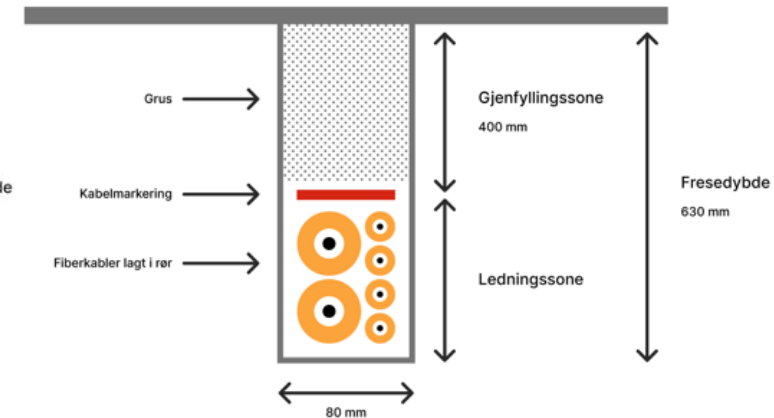
Kabelgrøft - Maskingraving
