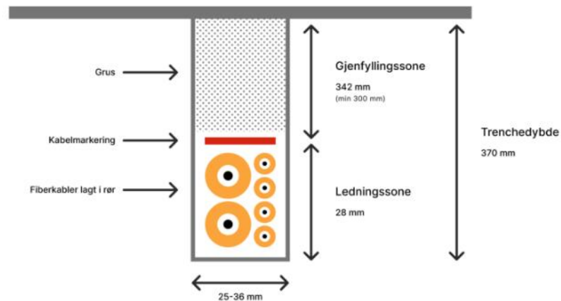
Kabelgrøft - Maskingraving
